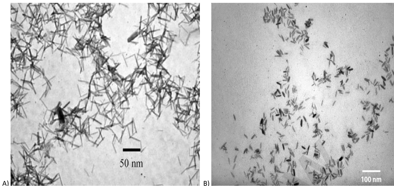
Figure 1: Photograph (transmission electron microscopy, TEM-125K, Selmi, Ukraine) of nanoparticles: A) \text{GdVO}_4:\text{Eu}^{3+} ; B) \text{LaVO}_4:\text{Eu}^{3+} (25, 26).
